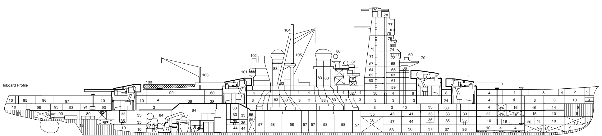
Inboard Profile
